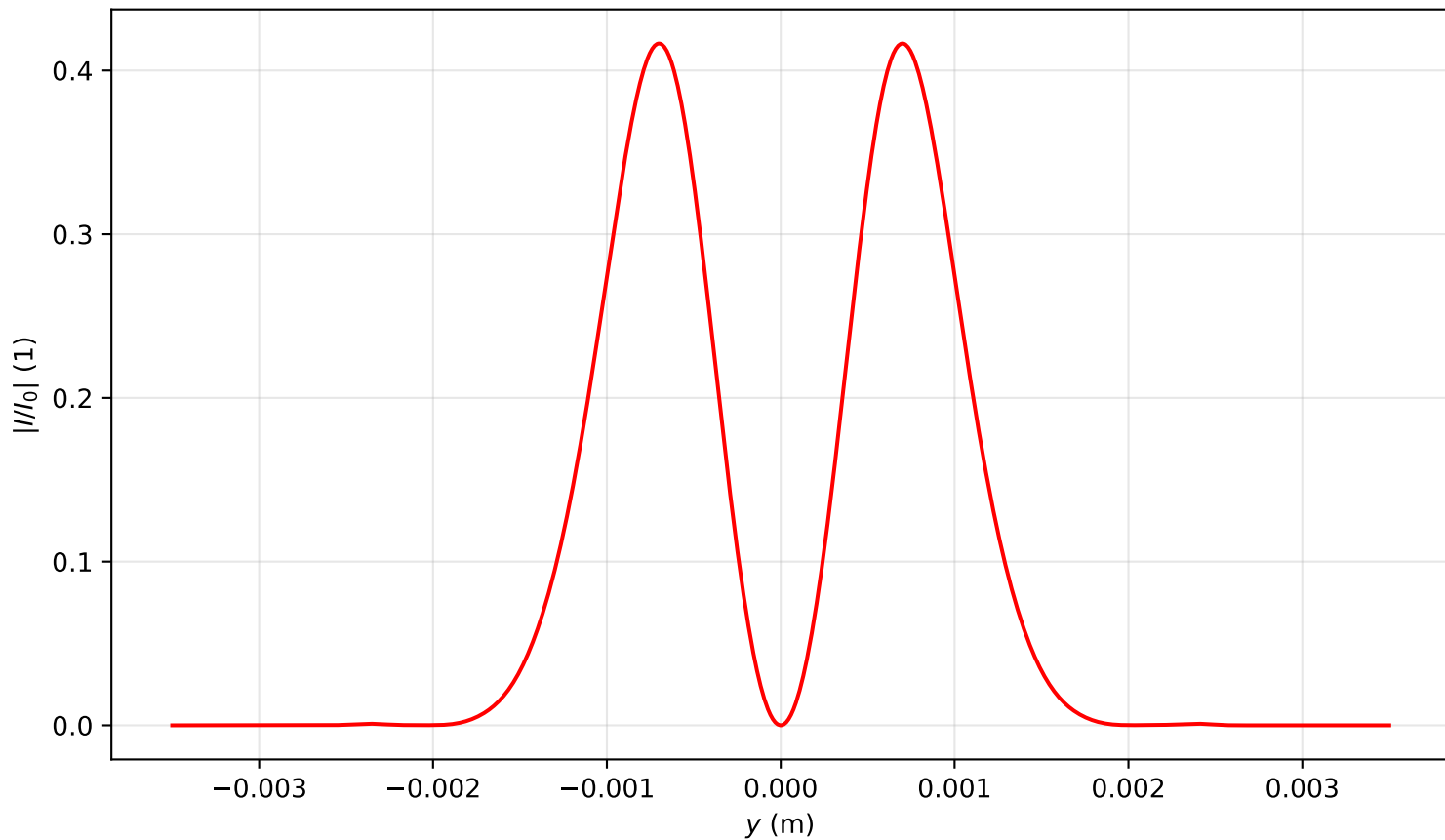
Intensity profile I(x=0, y, z=2.229)/I_0 , P_{in}=2.0P_{cr} , artificial time
